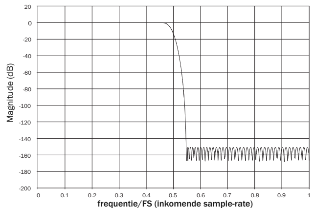
Frequentierespons lineaire fase filter
