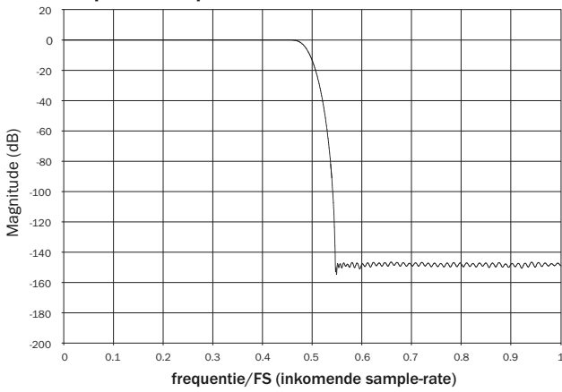
Frequentierespons minimale fase filter
