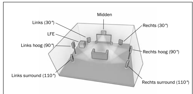
Configuratie 2 - 7.1 kanaals: L, C, R, LFE, Ls, Rs, Lhs, Rhs
