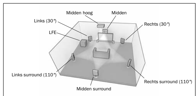
Configuratie 3 - 7.1 kanaals: L, C, R, LFE, Ls, Rs, Cs, Oh
